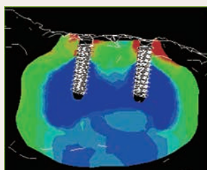
▲ Stress distribution of bone around the implant in a finite element analysis model using patient data.
